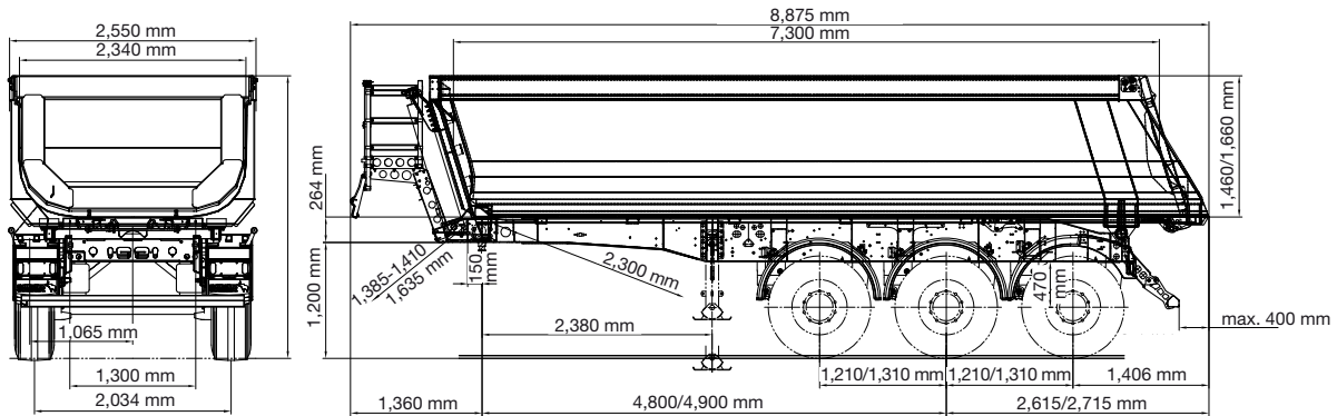
Three-axle rear tipper semitrailer design: steel body with chute and platform
